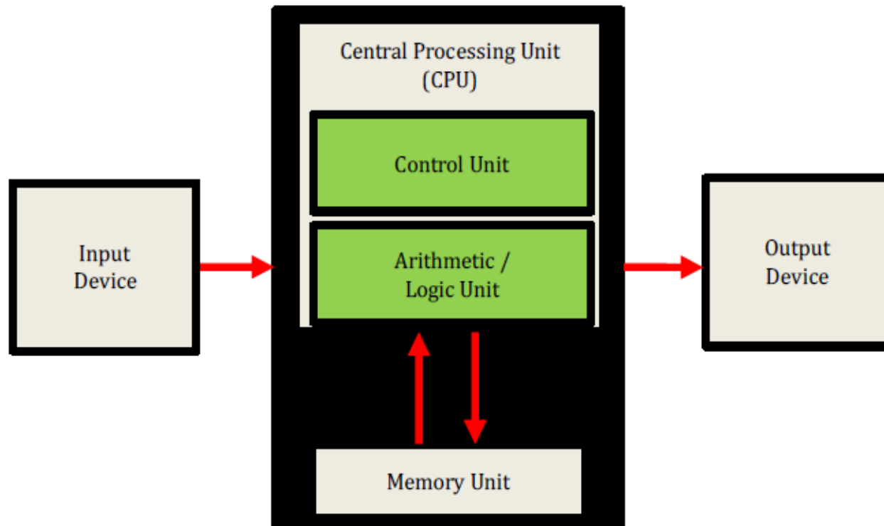
Figure 1. Comparison of high-level conventional and neuromorphic computer architectures. The so-called “von Neumann bottleneck” is the data path between the CPU and the memory unit. In contrast, a neural network based architecture combines synapses and neurons into a fine grain distributed structure that scales both memory (synapse) and compute (soma) elements as the systems increase in scale and capability, thus avoiding the bottleneck between computing and memory.
